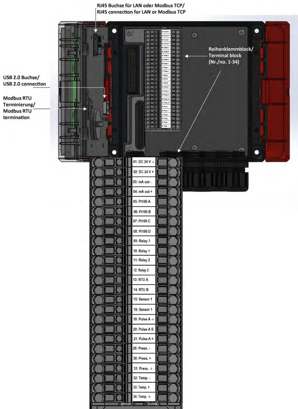
Illustration 43: Connection terminals GDR 1530 G2
